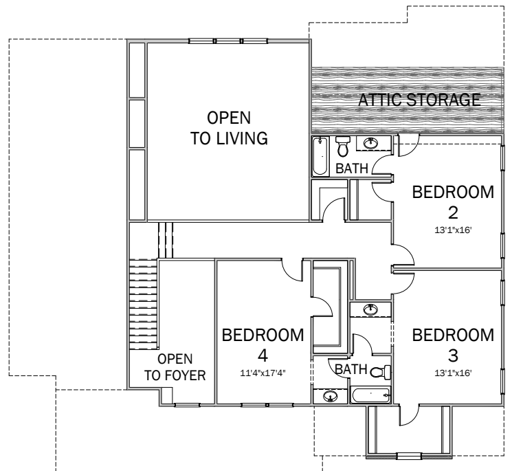
SECOND FLOOR
